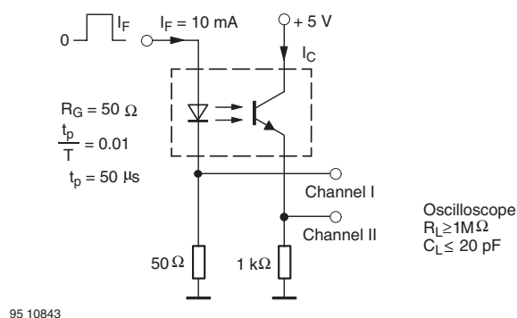
Figure 2. Test circuit, saturated operation
