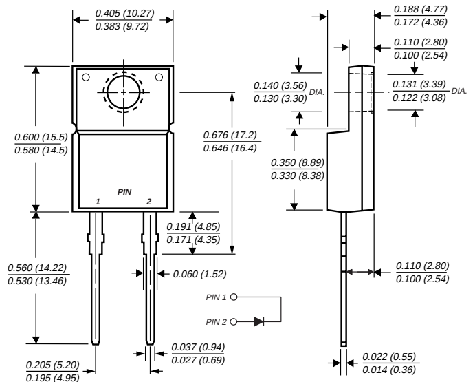
ITO-220AC (UGF8 Series)
