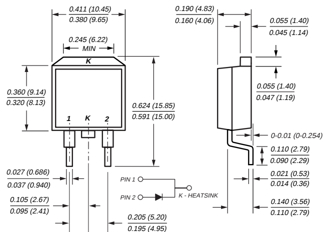
TO-263AB (UGB8 Series)
