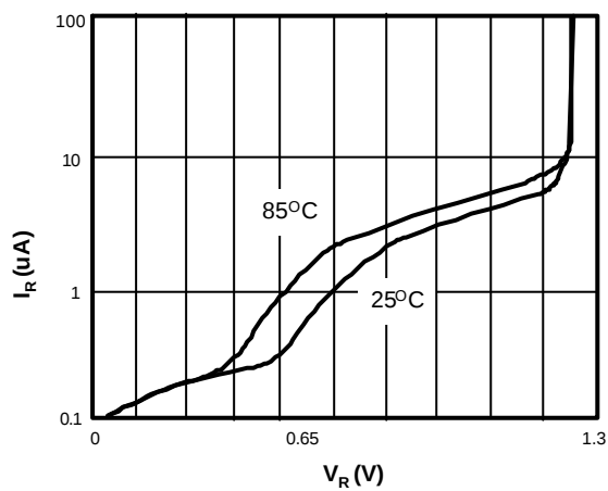
Reverse Characteristic
