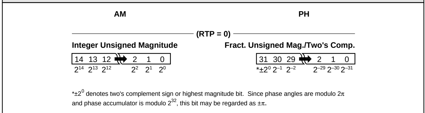
FIGURE 1A. INPUT FORMATS
