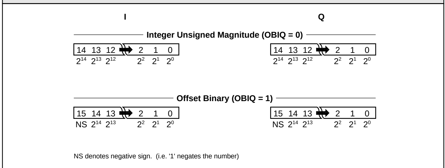
FIGURE 1B. OUTPUT FORMATS
