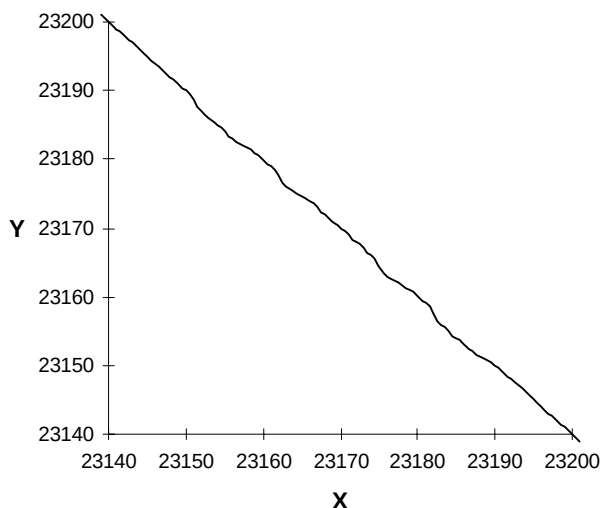
FIGURE 2. CIRCLE TEST RESULT NEAR 45° (16-BIT INTERNAL PROCESSOR)
