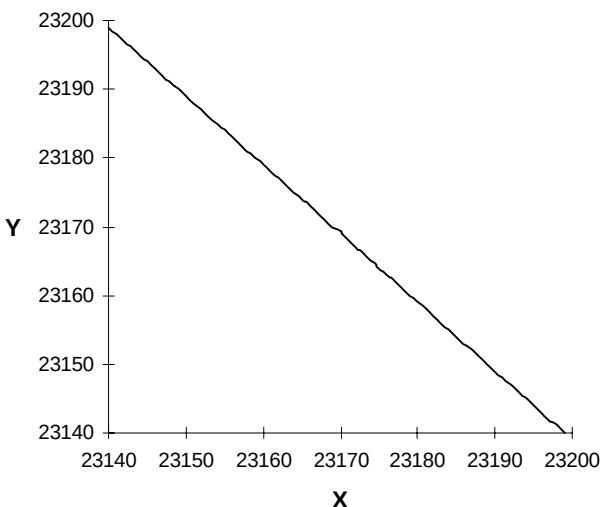
FIGURE 3. CIRCLE TEST RESULT NEAR 45° (24-BIT INTERNAL PROCESSOR)
