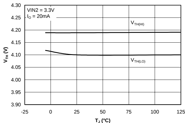
5V Detect Threshold Voltage vs. Junction Temperature
