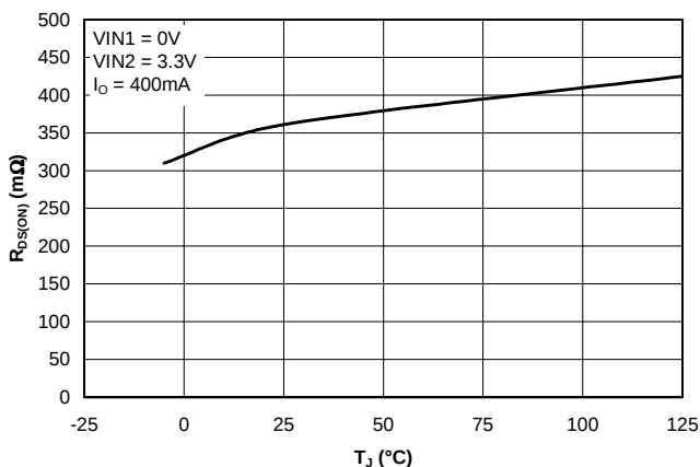
VIN2 Pass Device On Resistance vs. Junction Temperature
