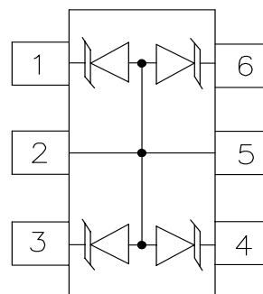
SOT23-6L (Top View)
