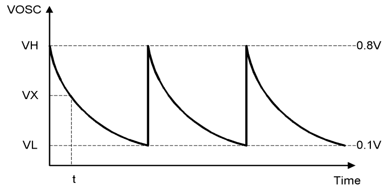
Figure 2 Oscillator Waveform
