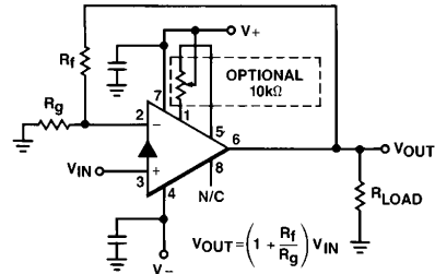
EL2020 Typical Non-Inverting Amplifier Characteristics
