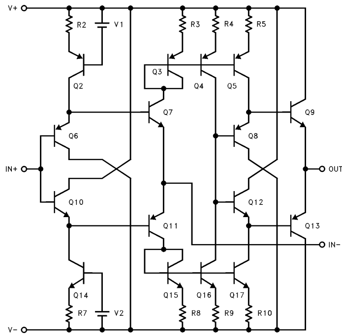
Simplified Schematic (per Amplifier)
