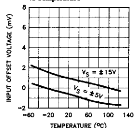
Input Offset Voltage vs Temperature
