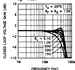
Voltage Gain vs Frequency A_V = -1 V_S = \pm 5V
