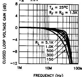
Voltage Gain vs Frequency A_V = +1 V_S = \pm 15V
