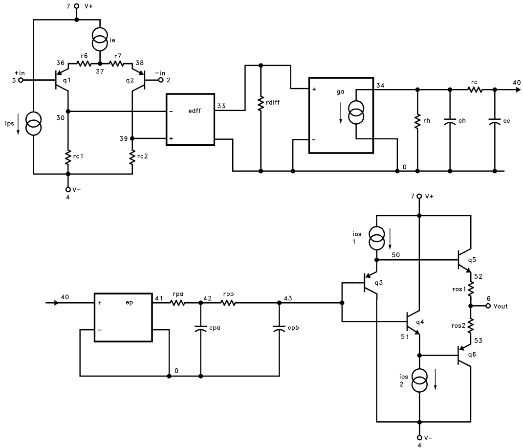
EL2245C/EL2445C Model
