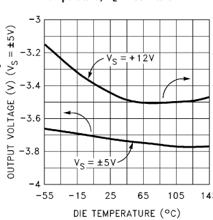
Negative Output Voltage Swing vs Die Temperature, R_L = 150Ω to GND
