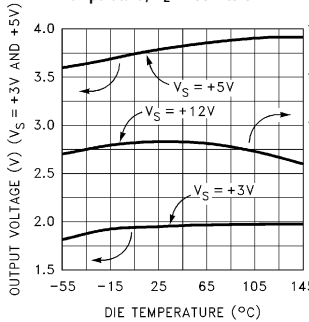
Positive Output Voltage Swing vs Die Temperature, R_L = 150Ω to GND
