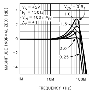
Non-Inverting Frequency Response vs Common Mode Voltage
