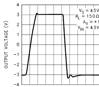
Large Signal Step Response, V_S = \pm 5V
