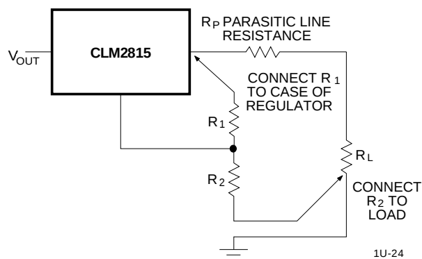
FIGURE 3. BASIC ADJUSTABLE REGULATOR
