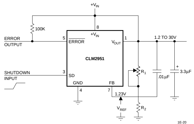
FIGURE 2. ADJUSTABLE REGULATOR
