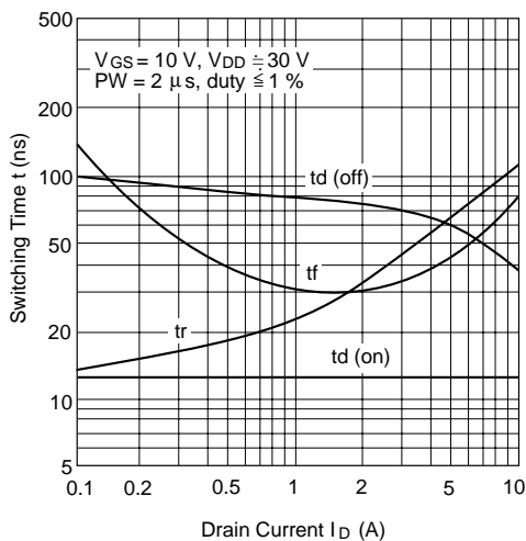
Switching Characteristics
