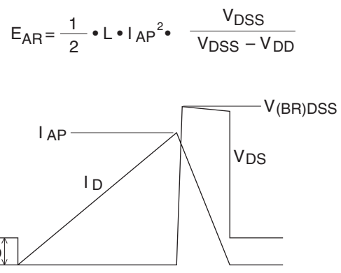
Avalanche Waveform
