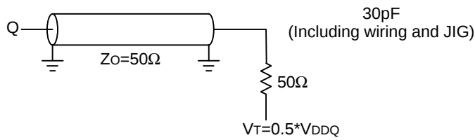
Fig.4 Output load
