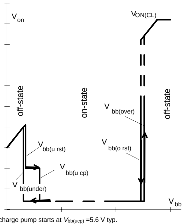
Figure 7a: Overvoltage:
