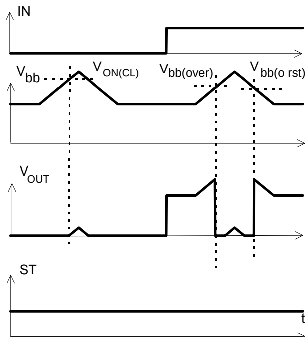
Figure 7a: Overvoltage:
