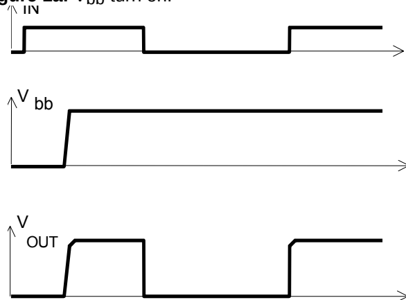
Figure 1a: V_{bb} turn on:
