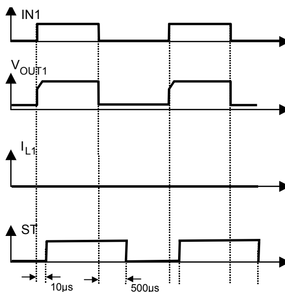
Figure 5a: Open load: detection in OFF-state, turn on/off to open load Open load of channel 1; other channels normal operation
