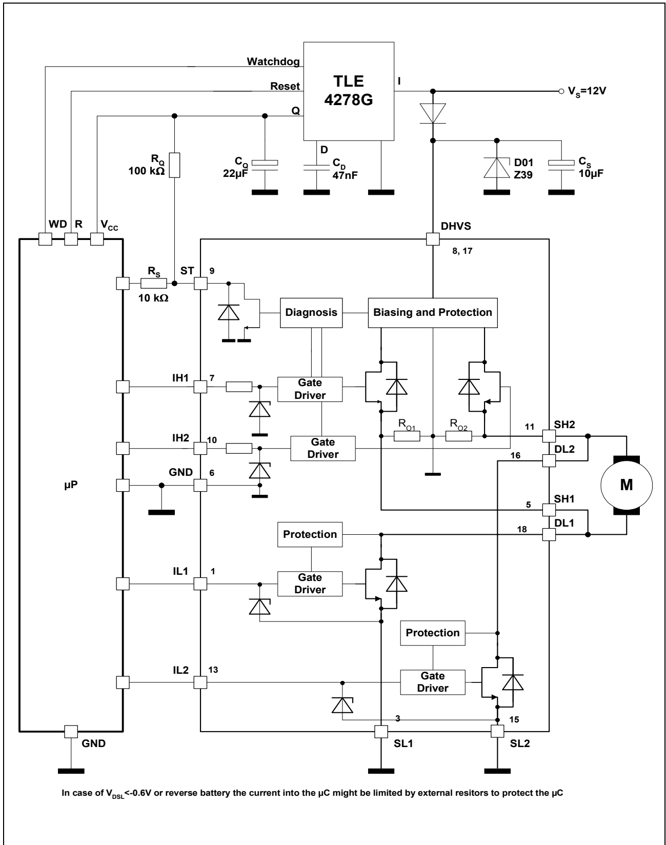
Figure 4 Application Circuit
