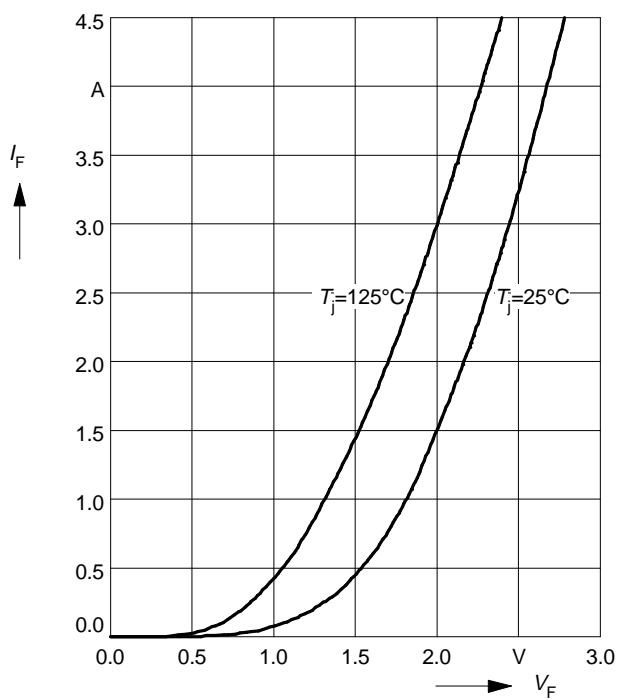
Forward characteristics of fast recovery reverse diode I_F = f(V_F) parameter: T_j
