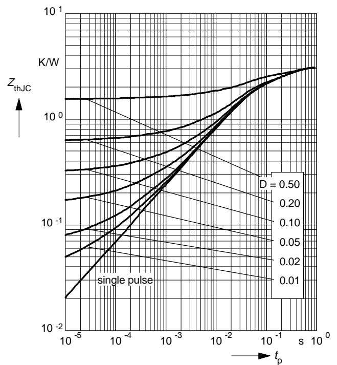
Transient thermal impedance Diode Z_{thJC} = f(t_p) parameter: D = t_p / T
