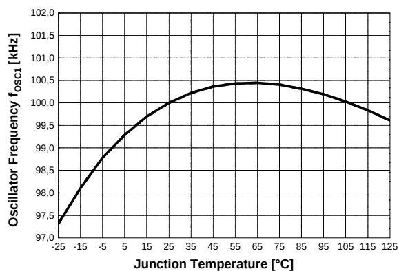
Figure 29 Oscillator Frequency f_{OSC1} vs. T_j
