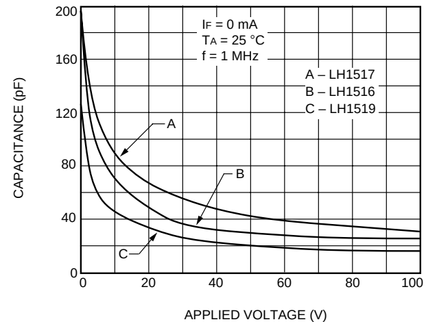
D. Switch Capacitance vs. Applied Voltage
