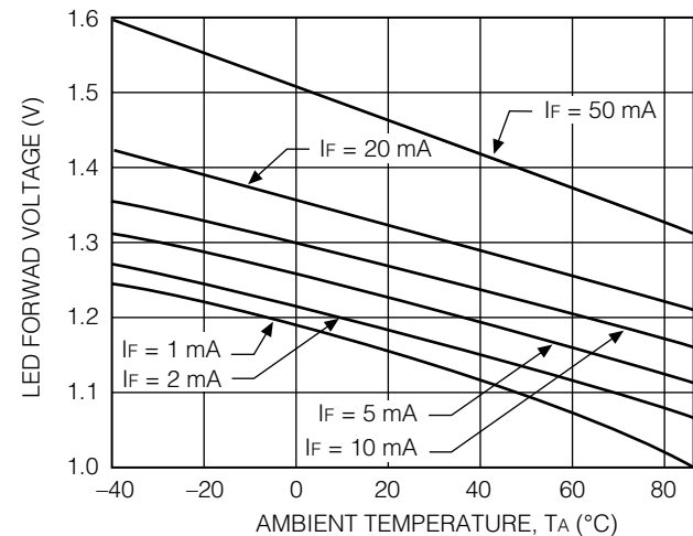
A. LED Voltage vs. Temperature
