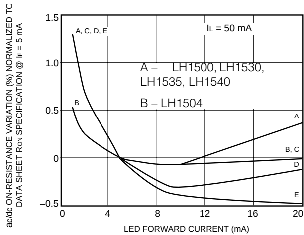
A. Variation in ON-Resistance vs. LED Current
