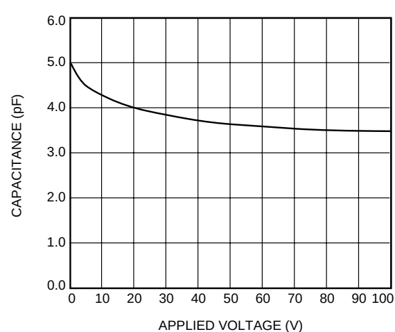
F. Switch Capacitance vs. Applied Voltage (LH1541)
