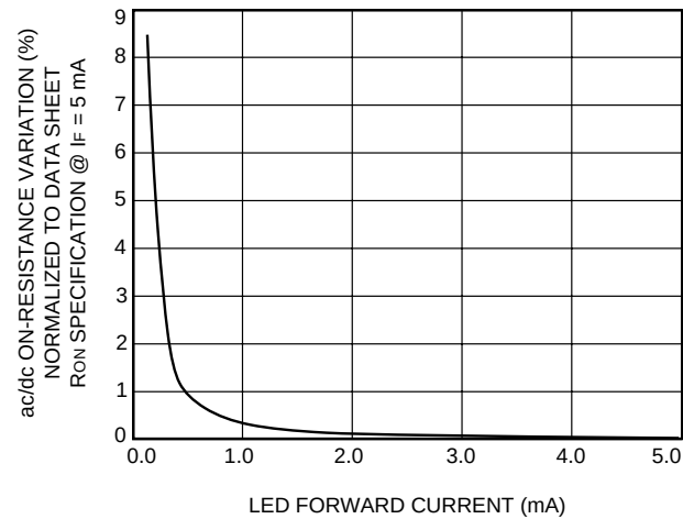
B. Variation in ON-Resistance vs. LED Current (LH1525)
