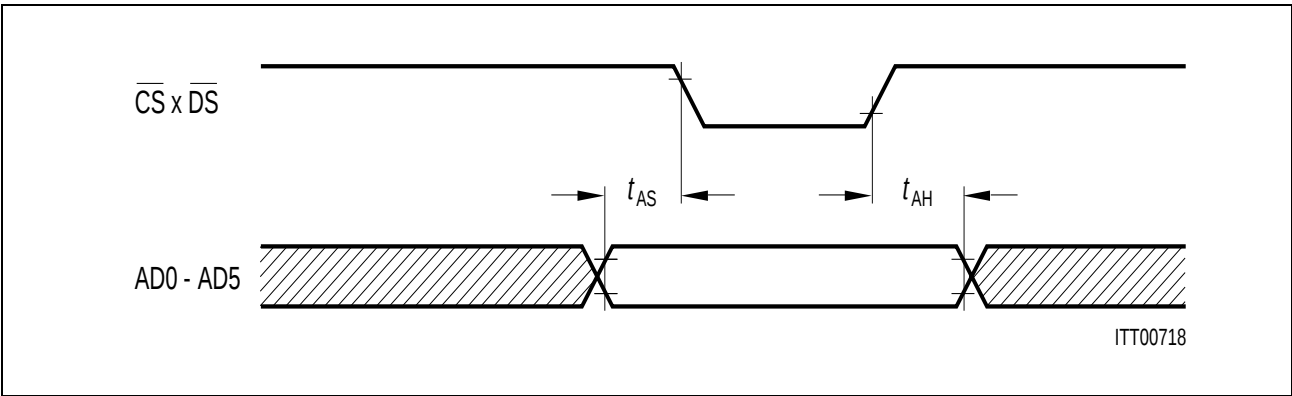
Figure 24 Address Timing
