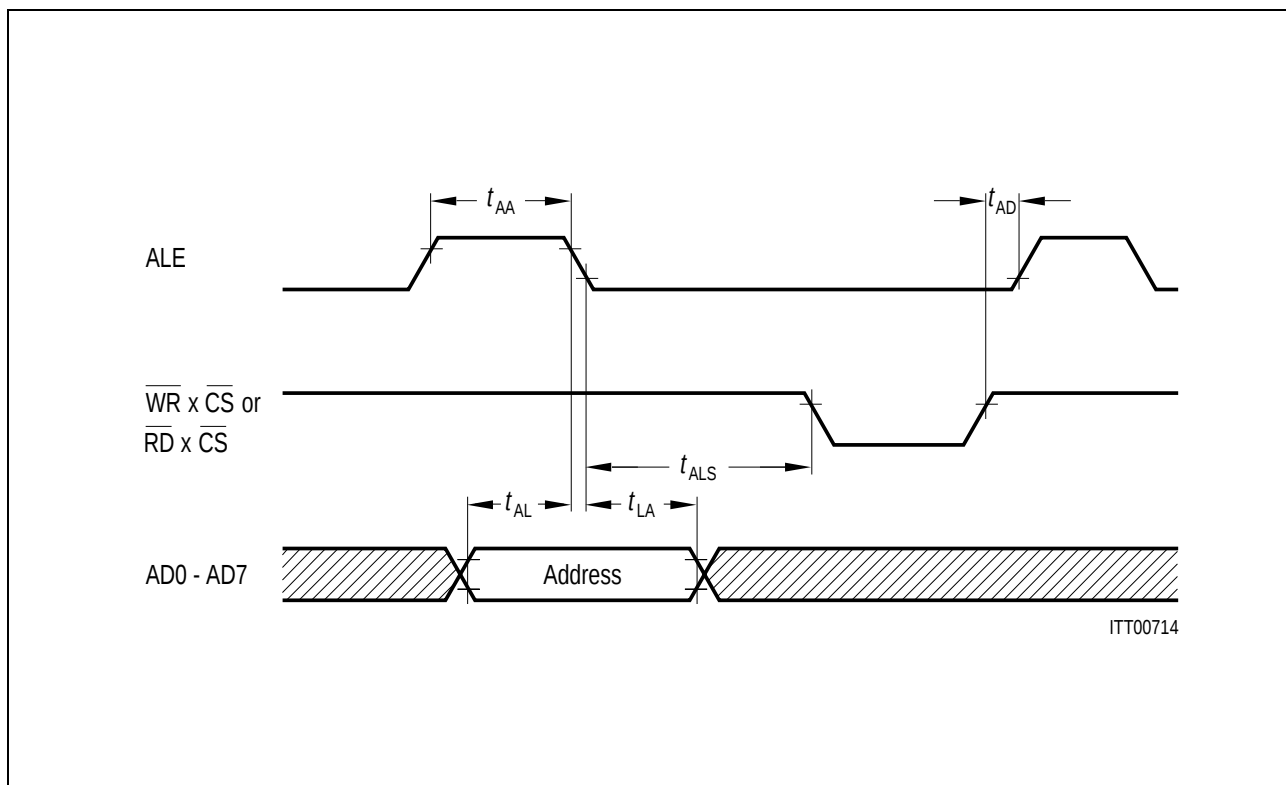
Figure 20 Multiplexed Address Timing
