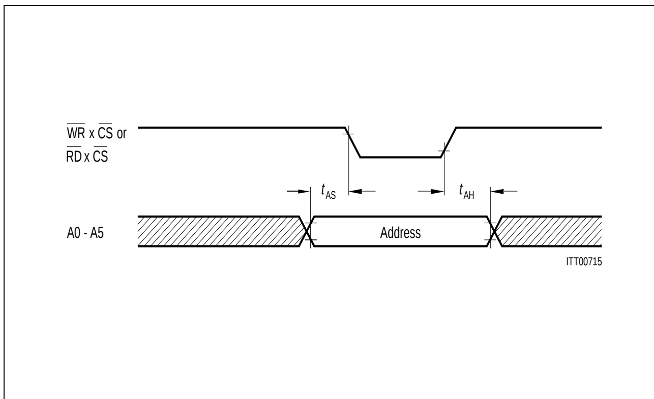
Figure 21 Demultiplexed Address Timing
