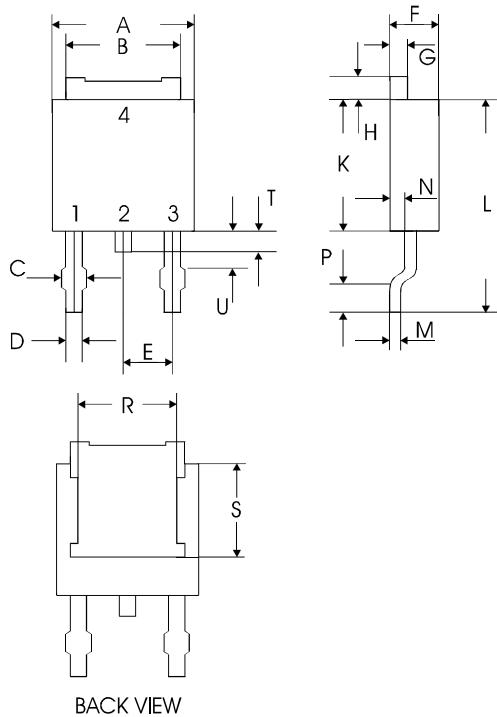
TO-252AA (DPak)
