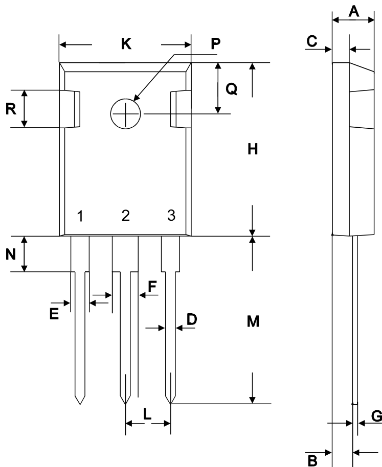
TO-247AC
