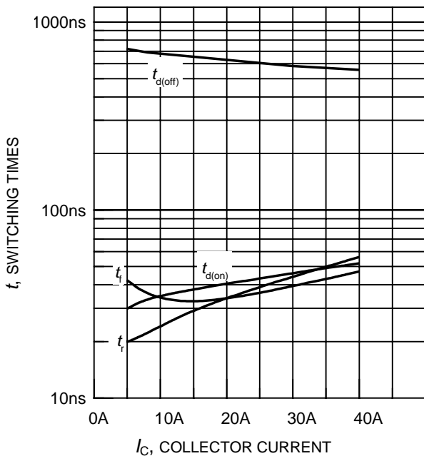
Figure 9. Typical switching times as a function of collector current (inductive load, T_j = 150^\circ\text{C} , V_{CE} = 800\text{V} , V_{GE} = +15\text{V}/0\text{V} , R_G = 33\Omega )
