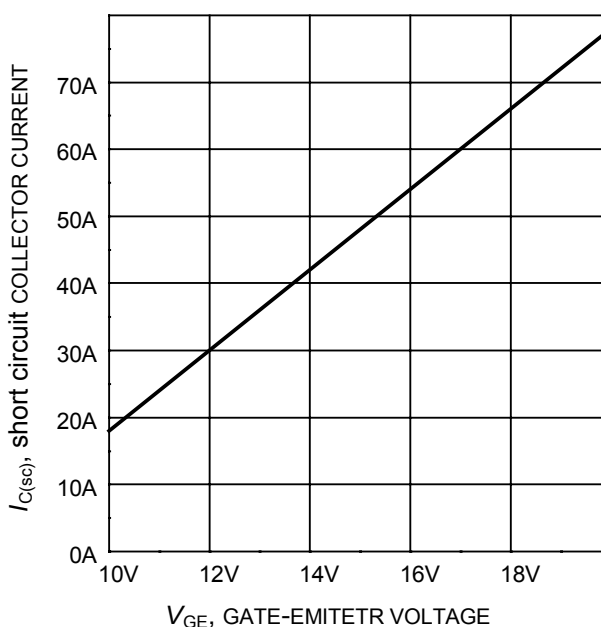
Figure 20. Typical short circuit collector current as a function of gate-emittetr voltage ( V_{CE} \leq 400\text{ V} , T_J \leq 150^\circ\text{C} )
