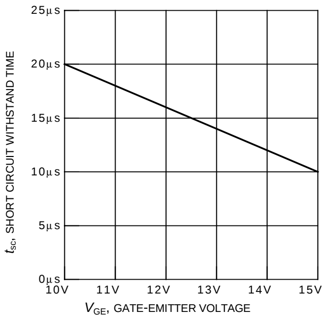
t_{sc} , SHORT CIRCUIT WITHSTAND TIME Figure 19. Short circuit withstand time as a function of gate-emitter voltage ( V_{CE} = 600V , start at T_j = 25^\circ C )
