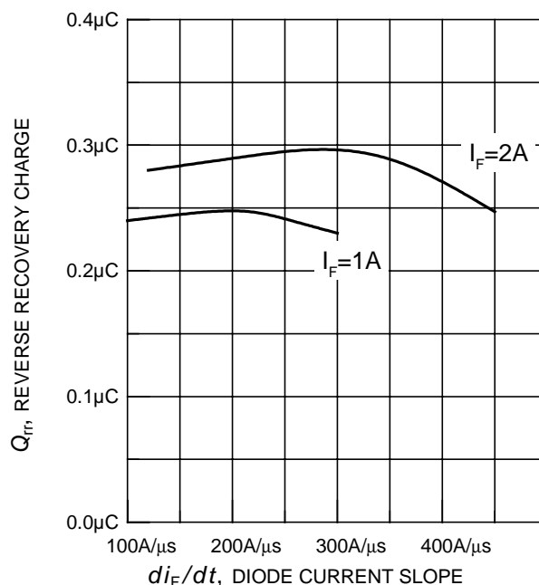
Figure 22. Typical reverse recovery charge as a function of diode current slope ( V_R = 800V , T_j = 150^\circ C , dynamic test circuit in Fig.E )
