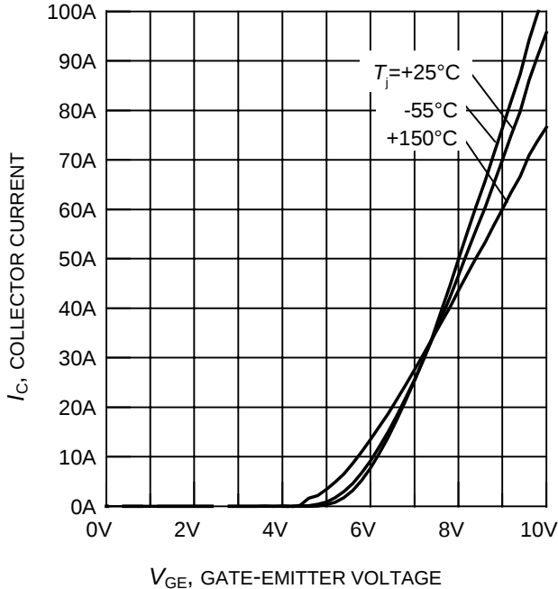
Figure 7. Typical transfer characteristics ( V_{CE} = 10V )
