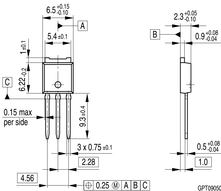
P-TO-251-3-1 (I-PAK)
