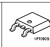
P-TO252-3-1
