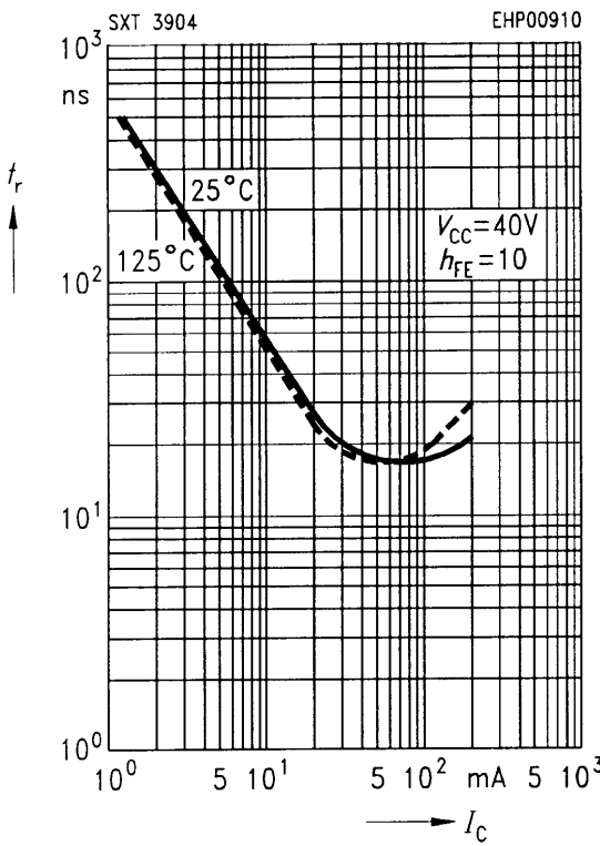
Rise time t_r = f(I_C)
