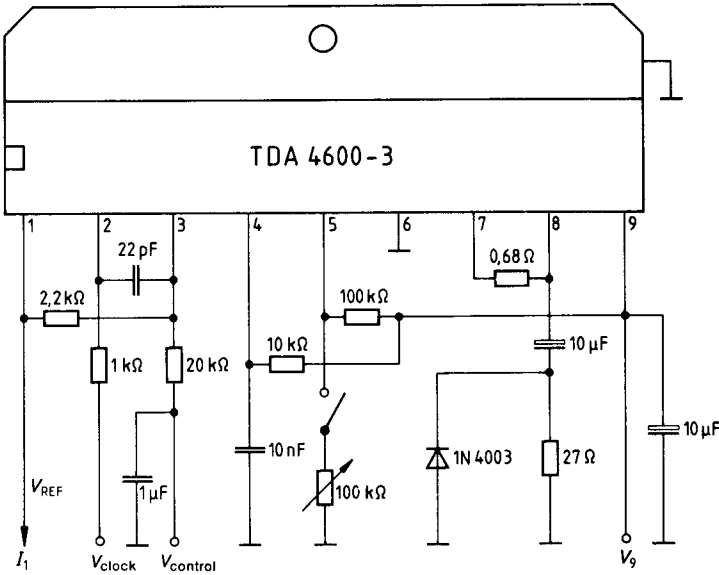
Measurement circuit 1
