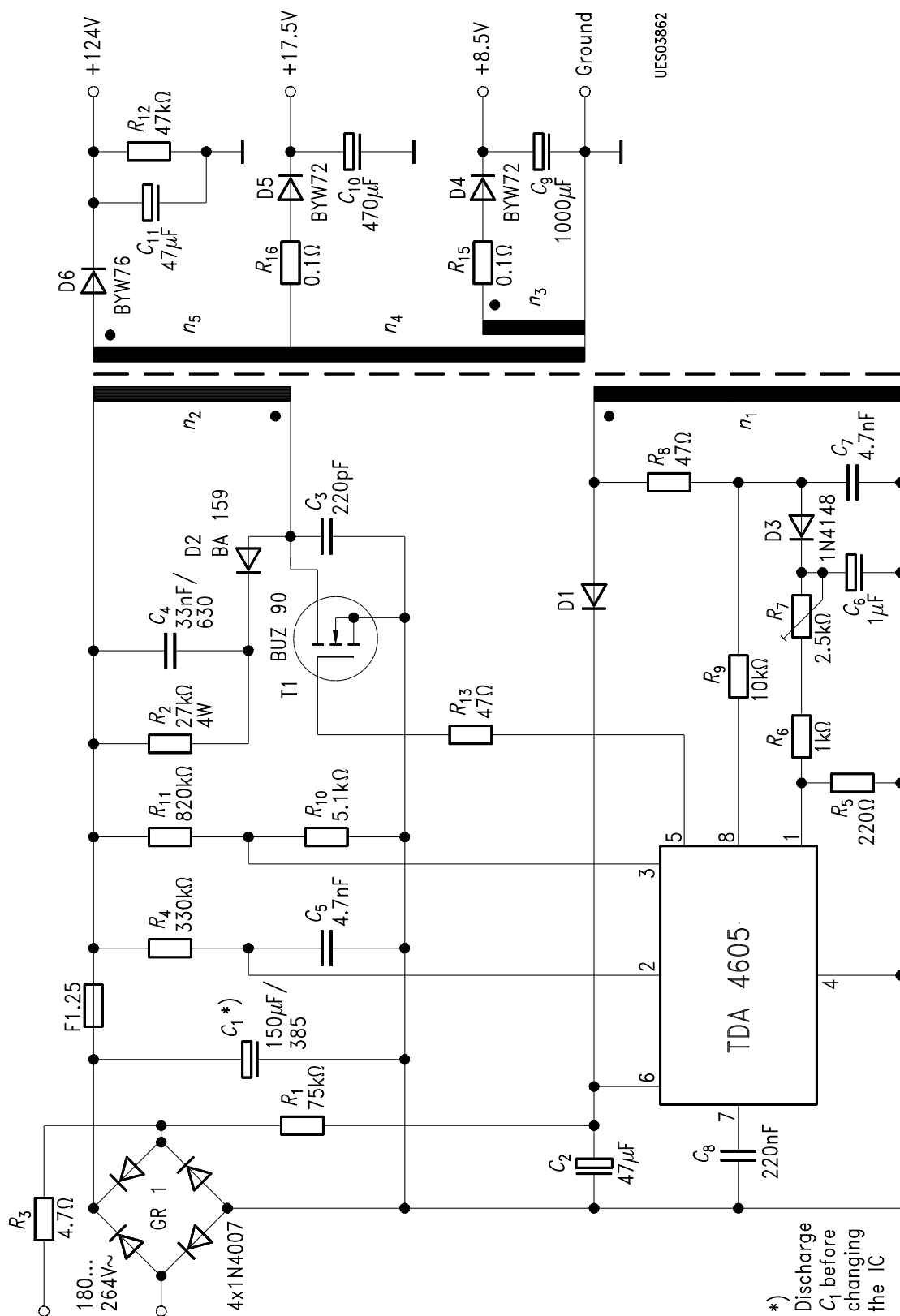
Application Circuit
