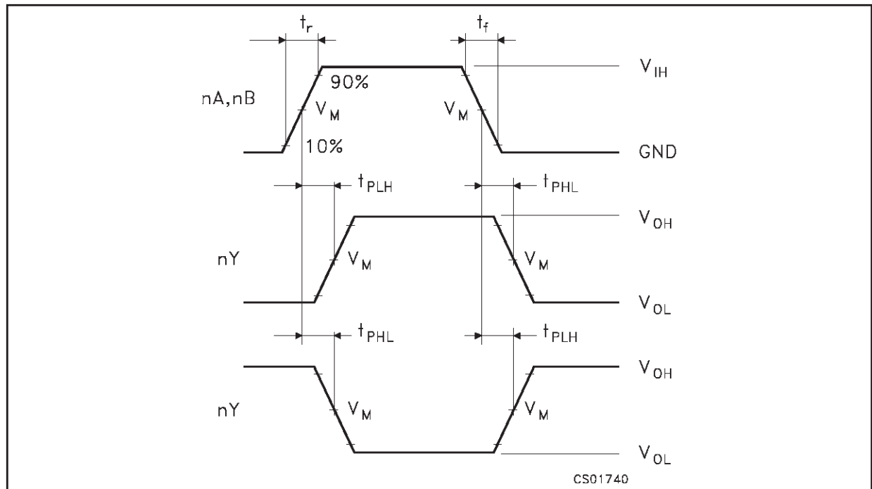
WAVEFORM: PROPAGATION DELAY ( f=1\text{MHz} ; 50% duty cycle)
