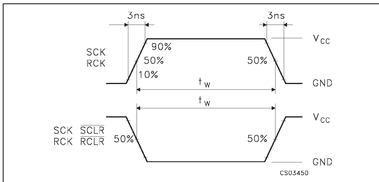
WAVEFORM 2: MINIMUM PULSE WIDTH ( f=1\text{MHz} ; 50% duty cycle)
