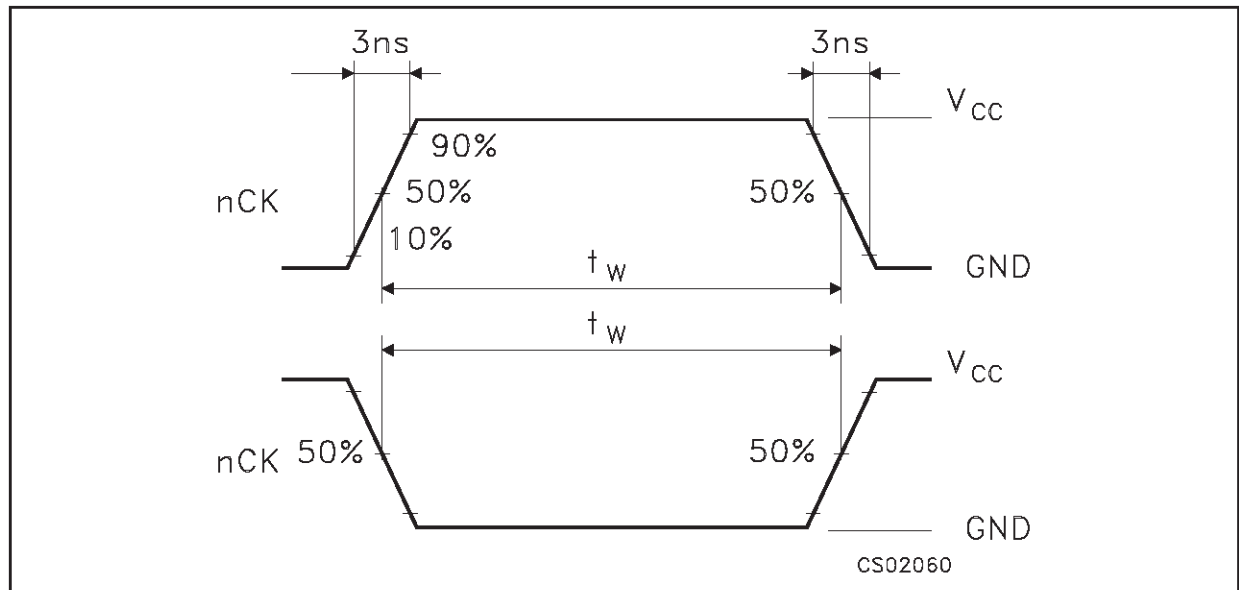
WAVEFORM 3 : CLOCK PULSE WIDTHS ( f=1\text{MHz} ; 50% duty cycle)
