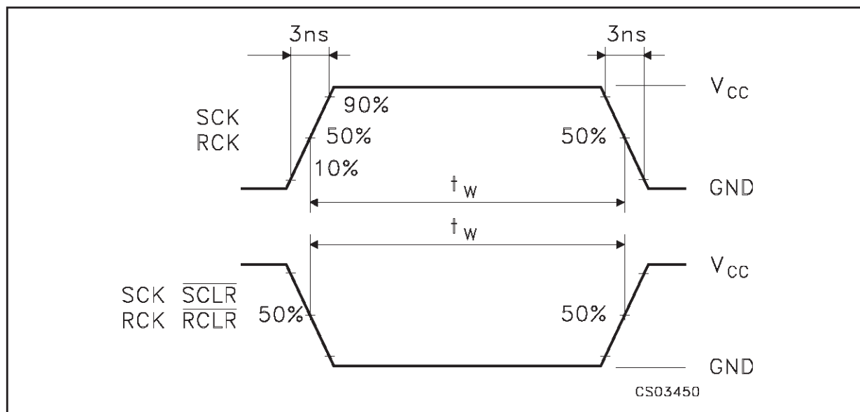
WAVEFORM 2: PULSE WIDTH (f=1MHz; 50% duty cycle)
