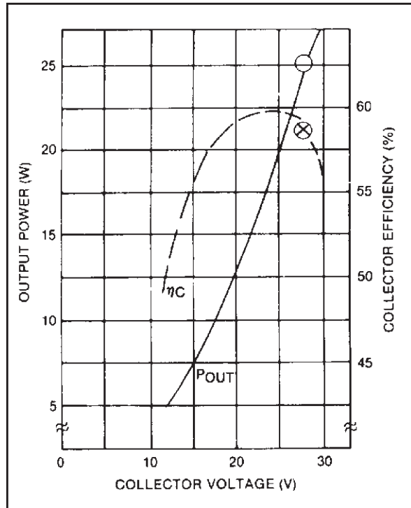
Output Power &amp; Collector Efficiency vs Collector Voltage
