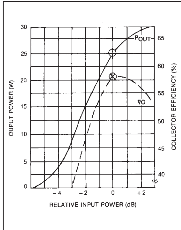
Output Power &amp; Collector Efficiency vs Input Power
