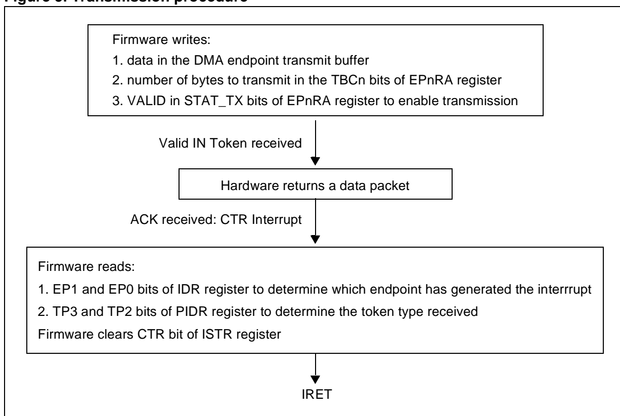
Figure 5. Transmission procedure
