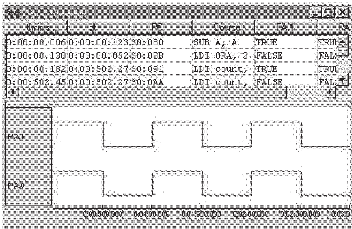
Figure 21. Trace window
