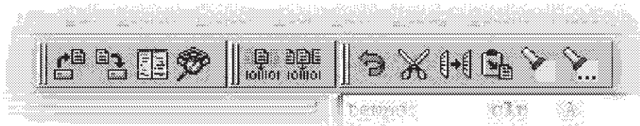
Figure 5. Editing toolbar
