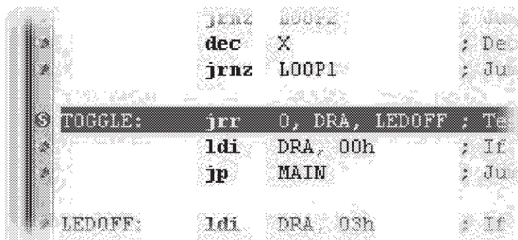
Figure 11. Set breakpoint
