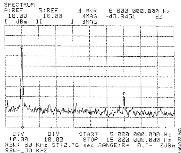
Figure 23 : Z = 470\Omega
