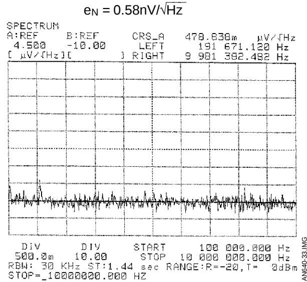
Figure 33 : e_N ( e_N = \frac{V_{OUT}}{G_V} , G_V = 59.3\text{dB} )
