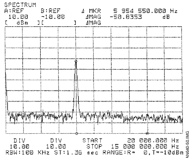
Figure 50 : V_{REC} = 5\text{V} , I_{REC} = 10\text{mA p-pk}
