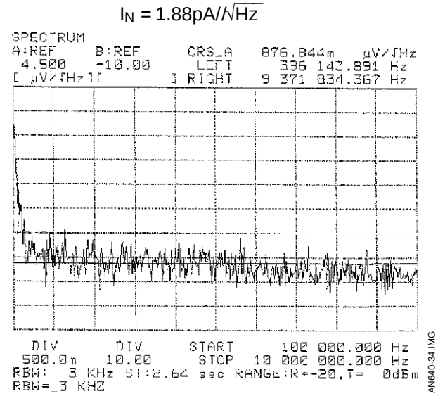
Figure 34 : I_N ( e_N = \frac{V_{OUT}}{G_V \cdot Z_{IN}} , Z_{IN} = 500\Omega )
