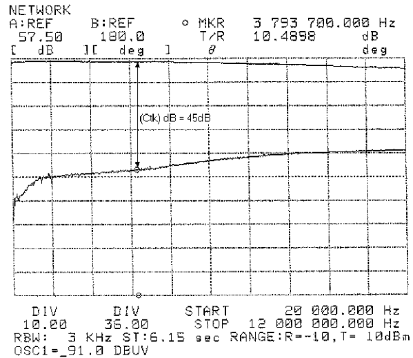
Figure 28 : H1SP - R_{IN} = 0
