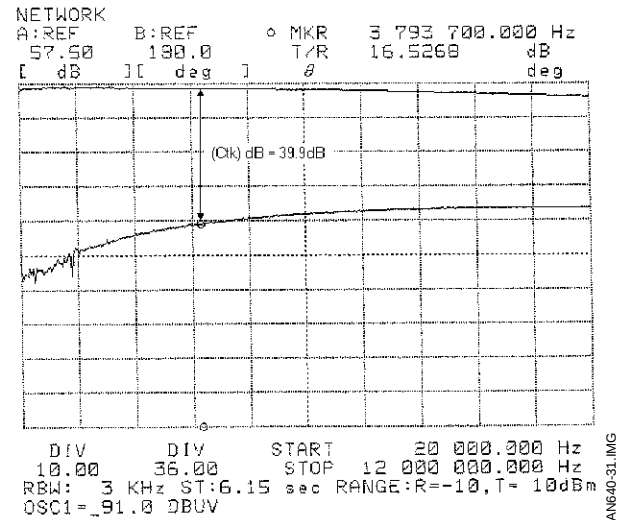
Figure 31 : H1SP - R_{IN} = \infty (open)
