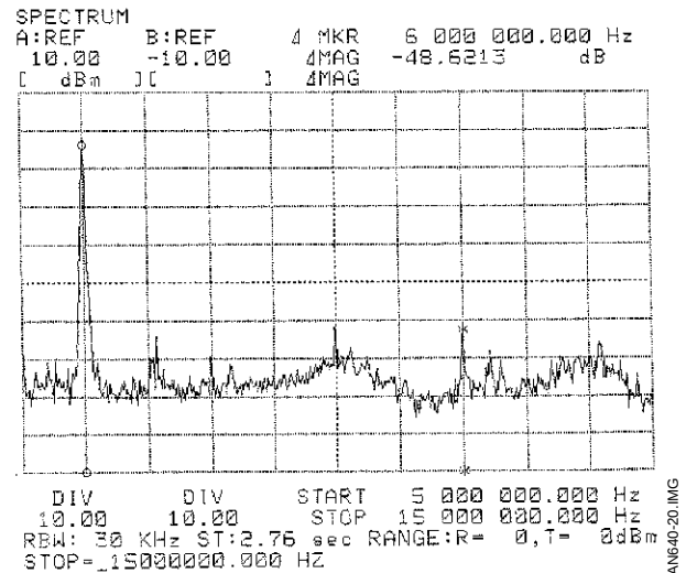
Figure 20 : Z = 470\Omega//100\text{pF}
