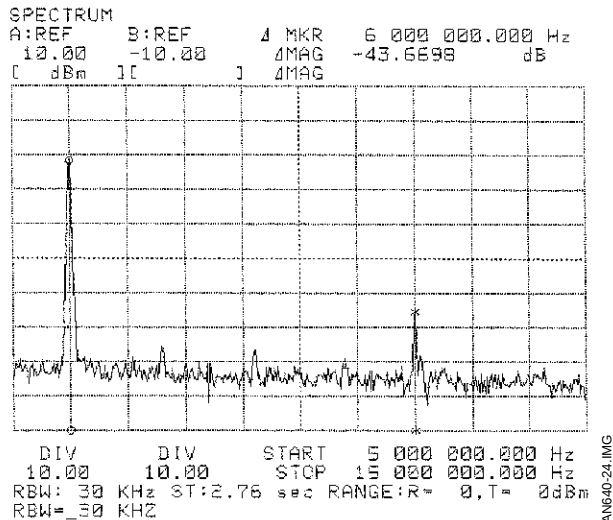
Figure 24 : Z = 470\Omega/100\text{pF}
