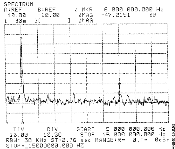
Figure 19 : Z = 470\Omega
