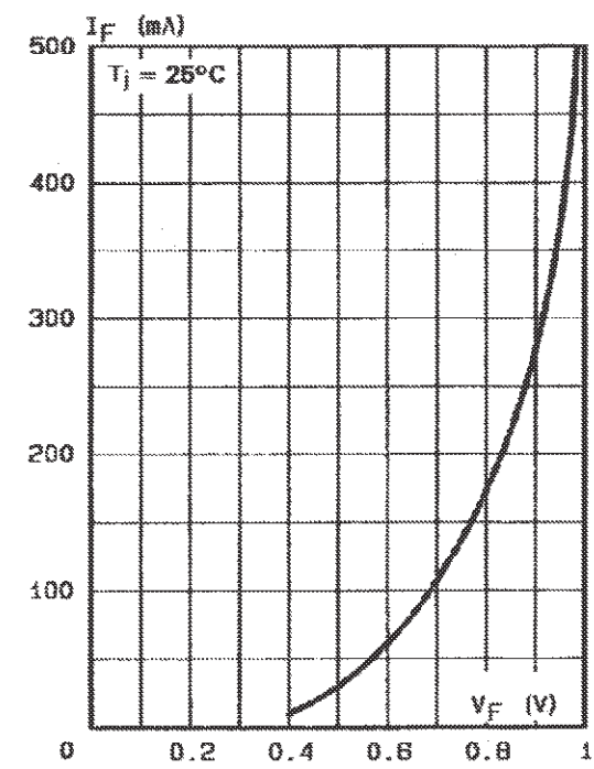
Figure 2. Forward current versus forward voltage (typical values).
