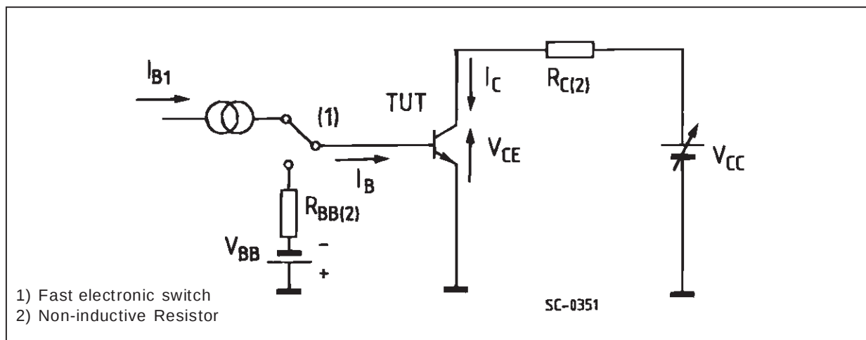
Turn-on Switching Test Circuit.
