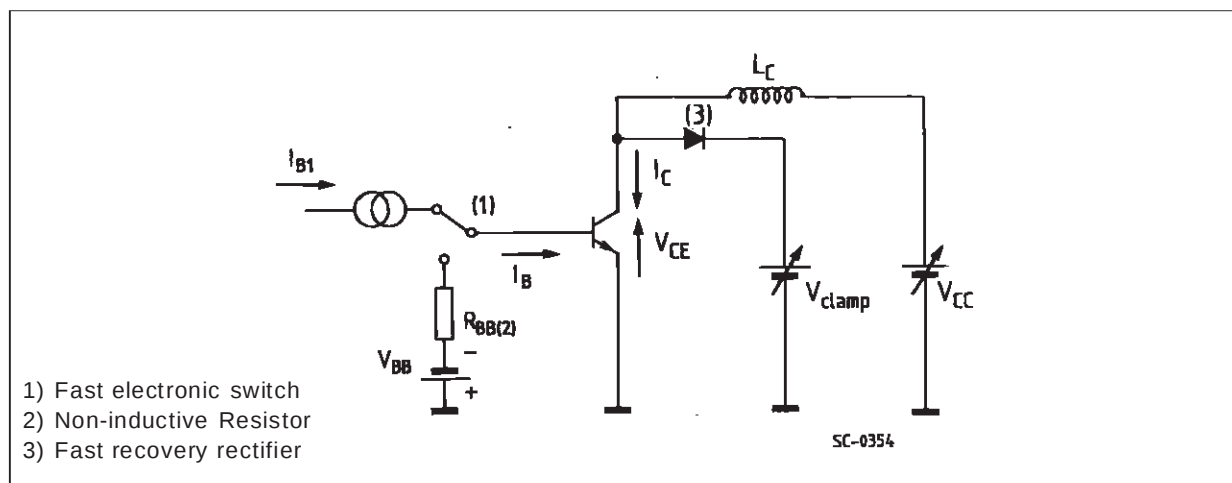
Turn-off Switching Test Circuit.
